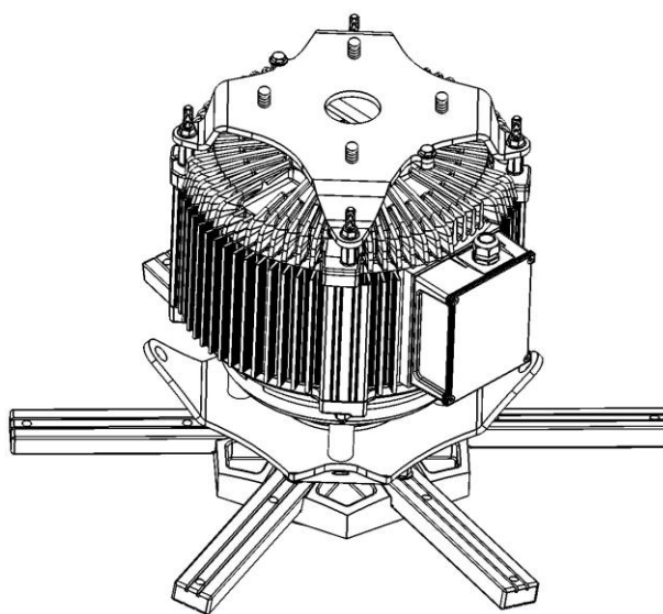
Motor Unit
